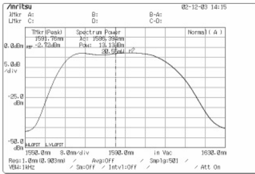
Output Power Spectrum
