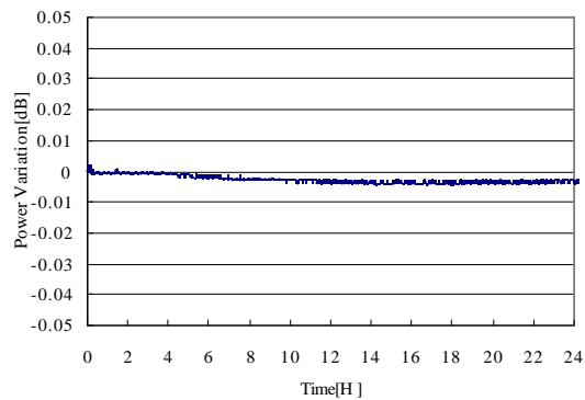
Total Output Power Stability
