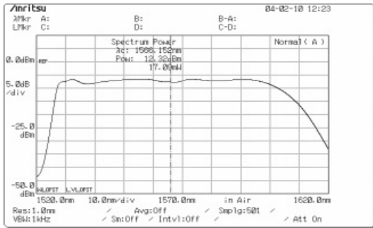
Output Power Spectrum
