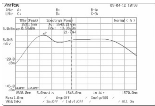
Output Power Spectrum
