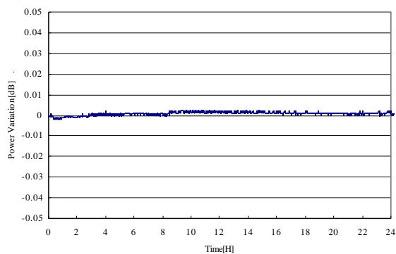
Total Output Power Stability
